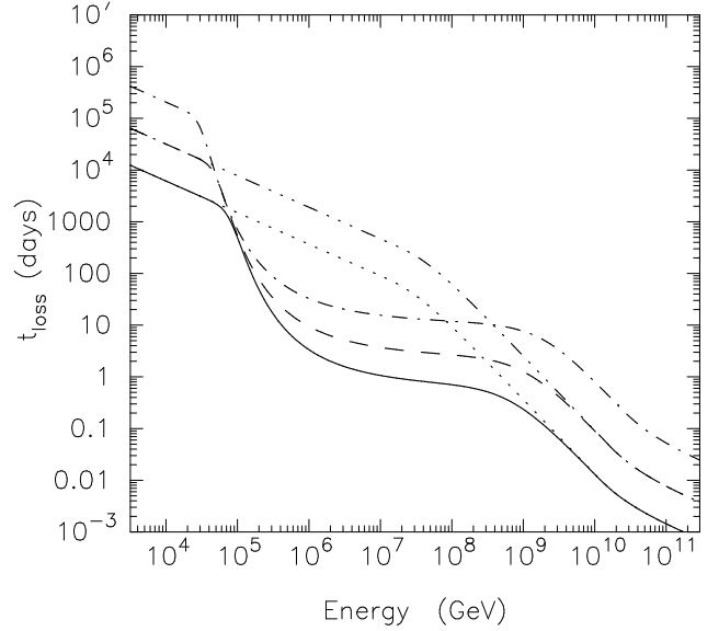
Fig. 1. Photomeson interaction energy loss time scale of protons, calculated for spectral fluxes observed from 3C 279 (see text) and t_{\text{var}} = 1 d, assuming 3 different Doppler-factors for the jet: \delta = 7 (solid curve), \delta = 10 (dashed curve), and \delta = 15 (dot-dashed curve). The dotted and triple-dot-dashed curves are calculated for \delta = 7 and \delta = 10 , respectively, when p\gamma interactions with the synchrotron radiation field alone are considered.
