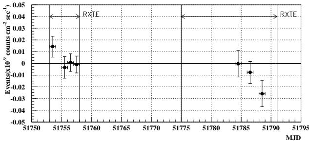
Fig. 4. The night by night number of excess events for PKS 2005–489. Vertical error bars indicate 1\sigma statistical errors.
