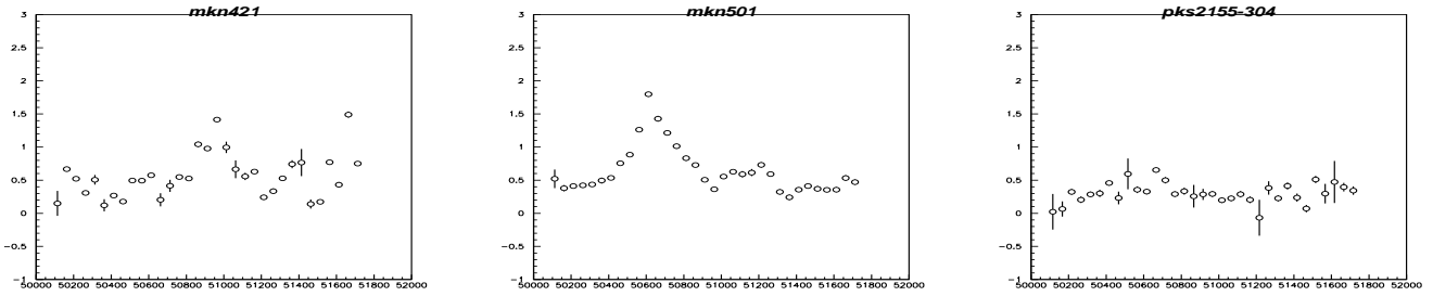
Fig. 1. Lightcurve of three interesting Blasers in our analysis. A possible periodicity with chance probability less than 10^{-3} is detected. Vertical axis is the count rate for each detector of ASM, horizontal axis is the observation time in unit of MJD. Data is binned in 50 day increments and selected with data points \geq 20 for clarity.
