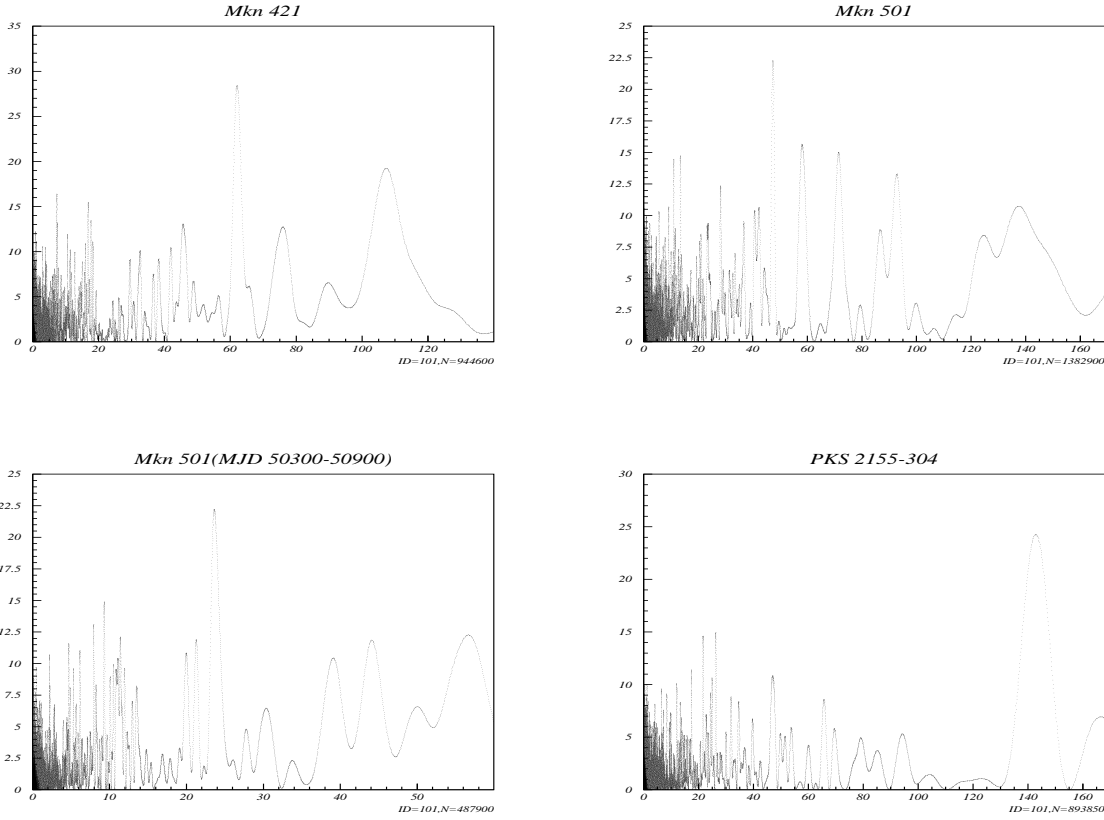
Fig. 2. Power spectra for Mkn 421, Mkn 501, Mkn 501 during MJD 50300-50900 (around the TeV flare time), PKS 2155-304. Low frequency components have been removed. This data has been obtained from no binning and S \geq 0 . Period less than T_{obs}/10 are shown. Vertical axis is power on a linear scale, horizon axis is periodicity in unit of day on a linear scale.
