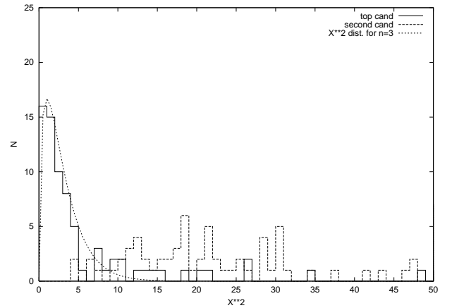
Fig. 1. \chi^2 distributions used for the data matching
