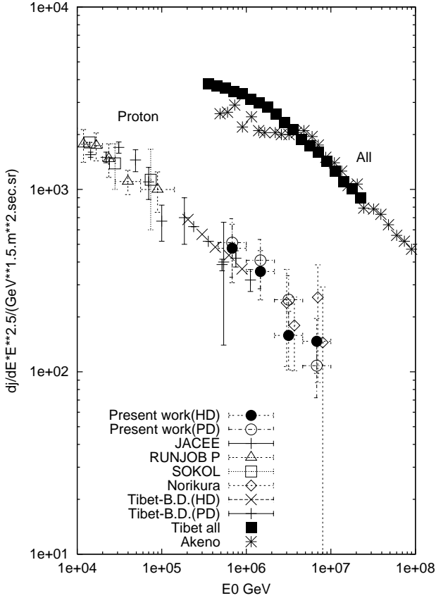
Fig. 2. Energy spectrum of protons in comparison with other experiments.
