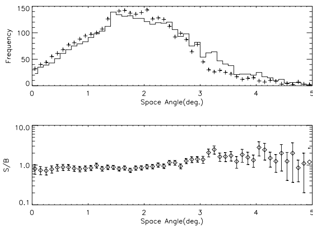
Fig. 3. The space angle distribution of two sets of background data taken on two different nights. The two data sets span the same hour angle range (upper panel). The lower panel shows the ratio of the two distributions as a function of space angle showing that when two background data-sets are compared no signal is seen adding credibility to the signal from the source reported here.
