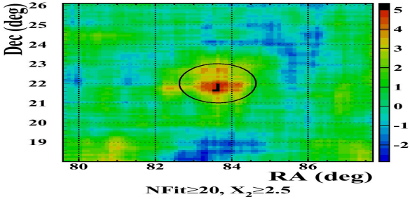
Fig. 8. Sky-map of the signal around the Crab. The colors represent the excess in sigma, with the scale at the right of the plot. The black circle is centered on the true Crab position.
