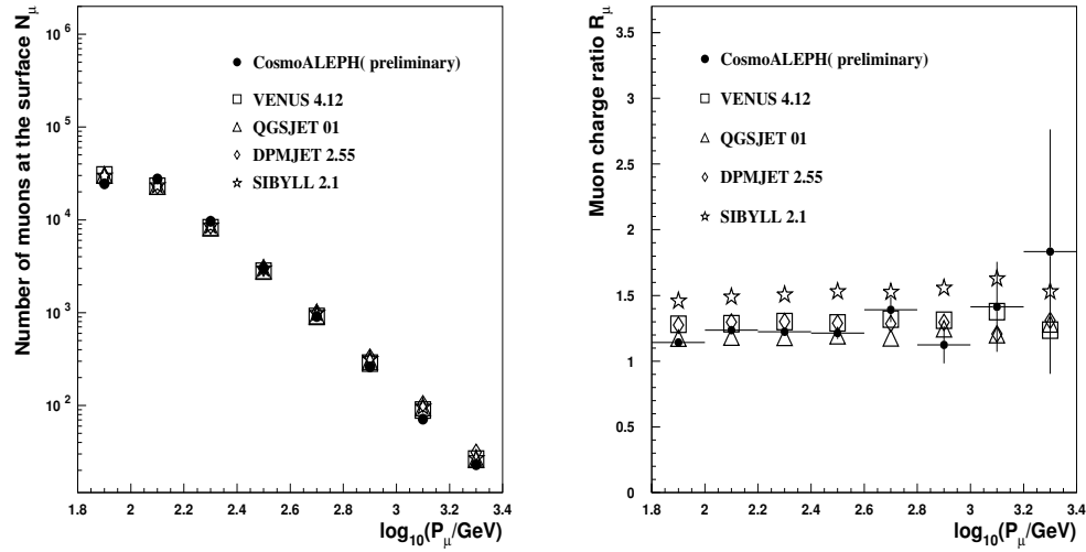
Figure 2. Number of vertical muons at the surface and their charge ratio compared with MC simulations based on different hadronic interaction models.
