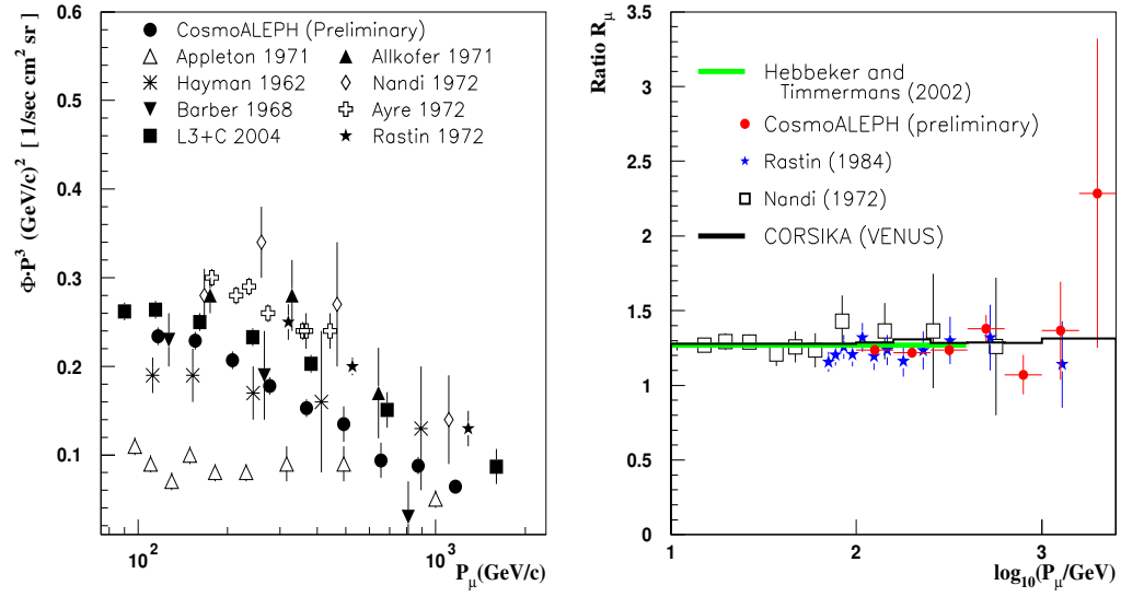
Figure 1. Momentum spectrum and charge ratio for vertical muons compared with other experiments[5, 17].
