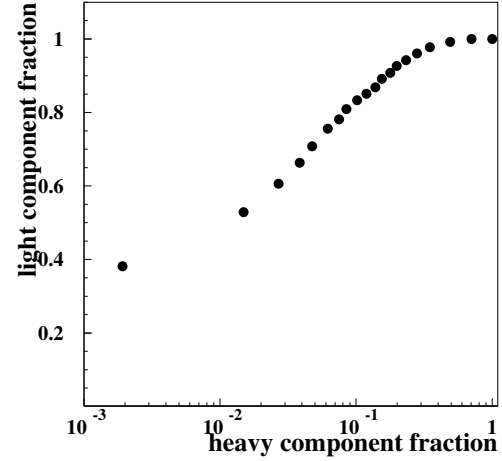
Figure 4. The fraction of the reconstructed light component as a function of the contamination from the heavy component.
