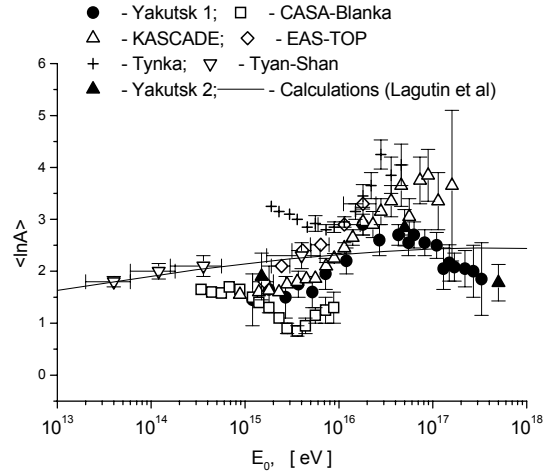
Figure 2b. Average mass of the primaries as a function energy. Experimental data in comparison with the calculations [4].
