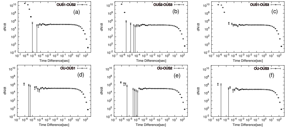
Figure 1. Time difference distributions for OUS-OUS and OU-OUS EAS array combinations: (a)OUS1-OUS2 ,(b)OUS2-OUS3 ,(c)OUS3-OUS1 for about 100m baseline combinations and (d)OU-OUS1, (e)OU-OUS2, (f)OU-OUS3 for about 1000m baseline combinations.
