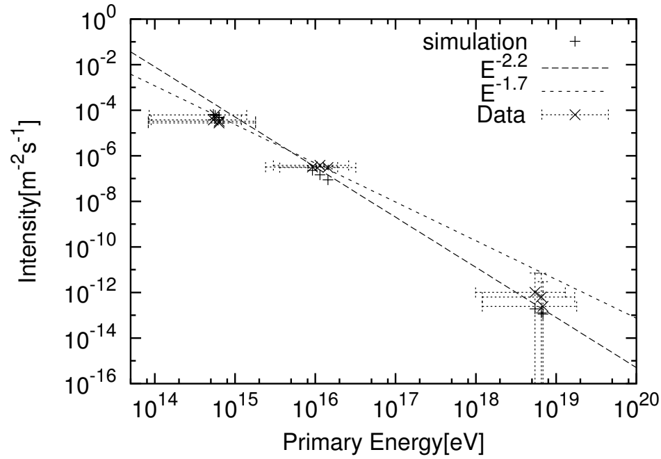
Figure 3. Integral cosmic ray energy spectrum with simulation results.
