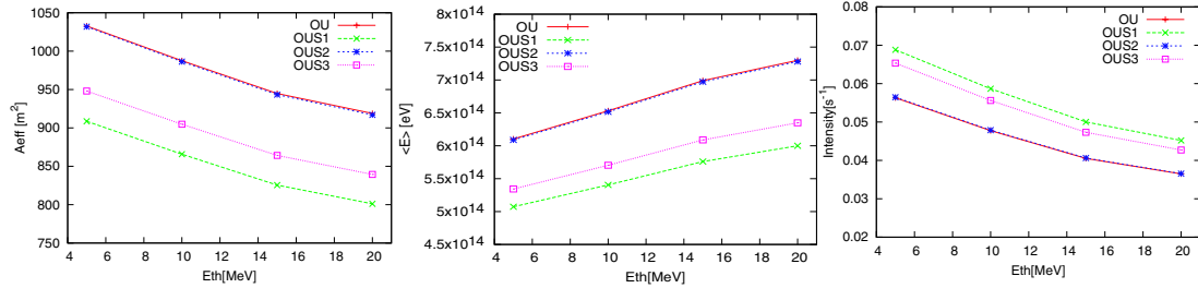
Figure 2. Threshold energy dependence of effective areas(left panel), average observed energy(center one) and primary cosmic ray intensity(right one).
