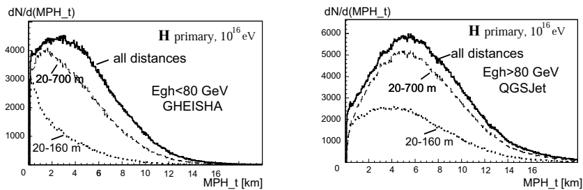
Figure 5. Distribution of true ( MPH_t ) muon production heights for two groups of grandmother hadron energies and three ranges of collecting distances.
