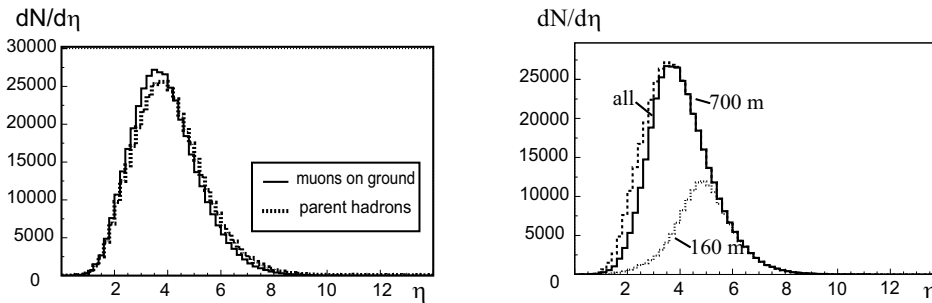
Figure 2. Pseudorapidity distributions for EAS muons. Comparison with the pseudorapidity of parent hadrons (left) and influence of the collecting distance to the core (right).
