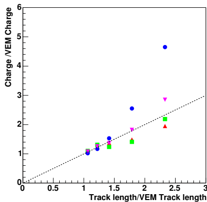
Figure 2. The points show for 5 different angles ( 20^\circ , 35^\circ , 45^\circ , 56^\circ and 70^\circ ) the charge measured in the 3 PMTs (triangle up, square, circle) as well as the total charge on the sum of the PMTs (triangle down), with respect to the track length in the tank. All quantities are normalized to the VEM corresponding values for comparison.
