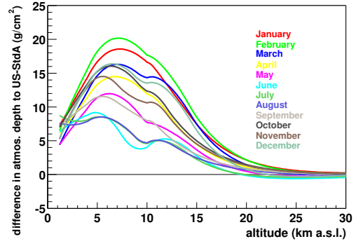
Figure 5. Profiles of atmospheric depth of the Malargüe Monthly Models in difference to the US-StdA.
