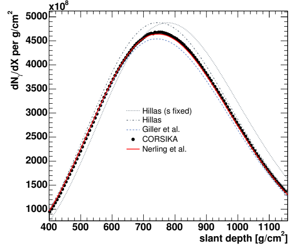
Figure 2. Longitudinal Cherenkov photon profile obtained by CORSIKA, different parameterisations (see text).
