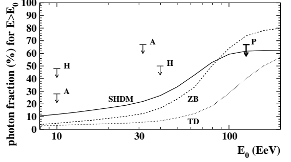
Figure 2. Upper limits on photon fraction (95% CL) from the present analysis (P) and previously from AGASA (A) [3] and Haverah Park (H) [11] compared to some predictions based on super-heavy dark matter (SHDM) [12], Z-bursts (ZB) and topological defect (TD) [13] models.
