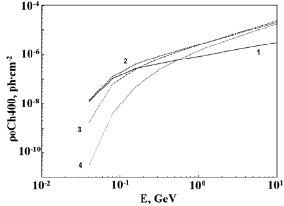
Figure 4. Dependence of the Cherenkov photon density at a distance of 400 m in the \gamma -induced showers from the shower core on energy E :
