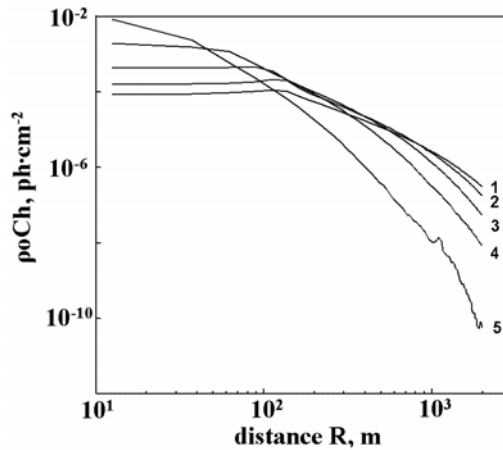
Figure 2. Lateral distributions of the Cherenkov photons for the \gamma -induced showers with energy of 10 GeV: 1 – 0 g/cm 2 , 2 – 200 g/cm 2 , 3 – 400 g/cm 2 , 4 – 600 g/cm 2 , 5 – 800 g/cm 2 .
