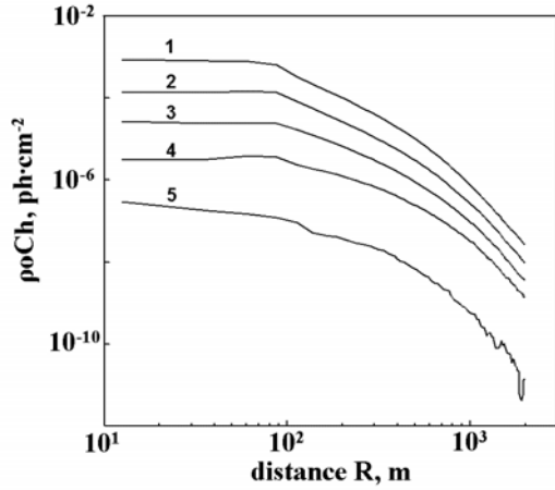
Figure1. Lateral distributions of the Cherenkov photons for the \gamma -induced showers from the depth of 500 g/cm 2 : 1 – 10 GeV, 2 – 2.51 GeV, 3 – 0.63 GeV, 4 – 0.16 GeV, 5 – 0.04 GeV.
