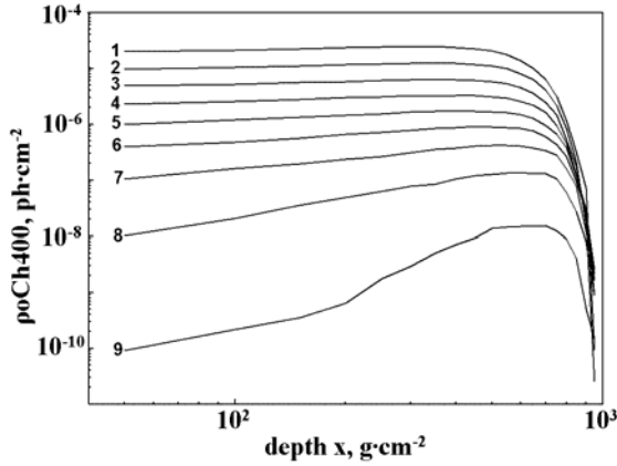
Figure 3. Dependence of the Cherenkov photon density at a distance of 400 m in the \gamma -induced showers from the shower core on depth x :
