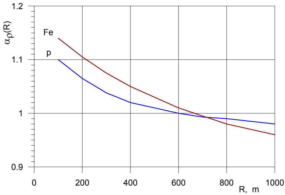
Figure 2 The dependence of \alpha_p(R) for p and Fe primaries (QGSJET model)
