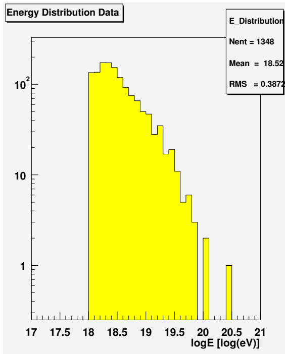
Figure 3. Energy distribution. Cosmic ray data.
