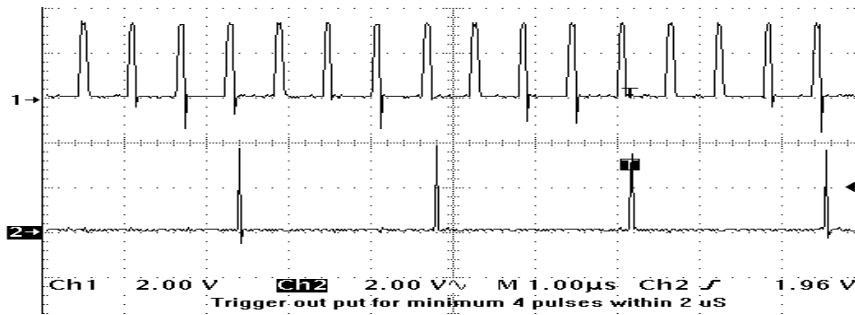
Fig5:Trigger out-put for minimum 4 pulses within 2 \mu S .
