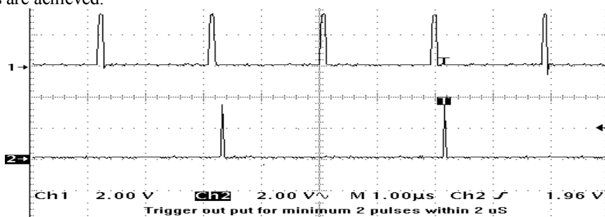
Fig4: Trigger out put for minimum 2 pulses within 2μS.
