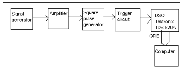
Fig3: Block Diagram of Testing of Trigger Circuit.
