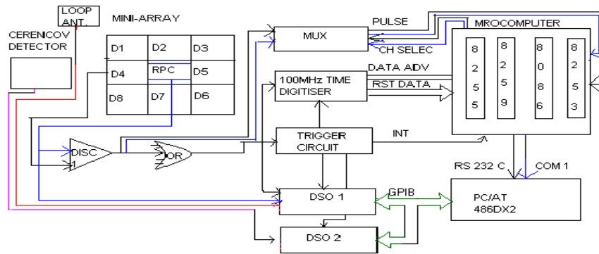
Fig1:Block Diagram of Experimental Set-up.
