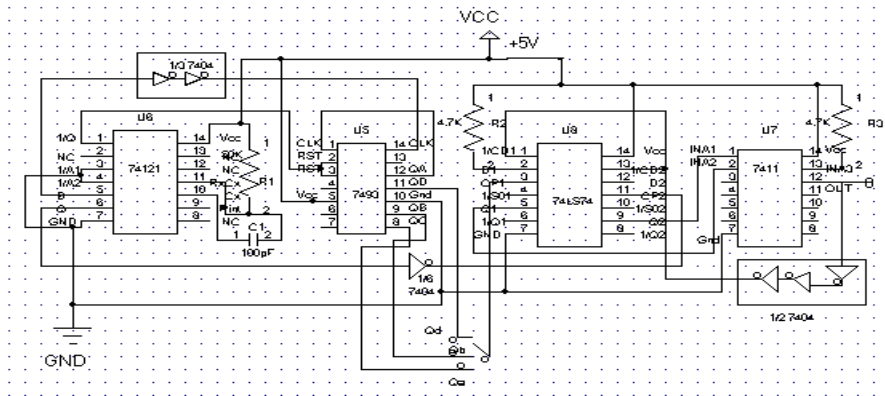
Fig2: Schematic Diagram of Trigger Circuit.
