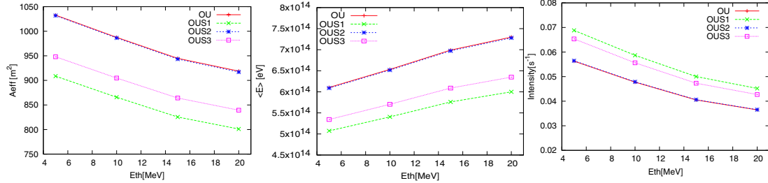
Figure 2. Dependence of effective areas(left panel), average observed energy(center one) and primary cosmic ray intensity(right one) on the threshold energy.
