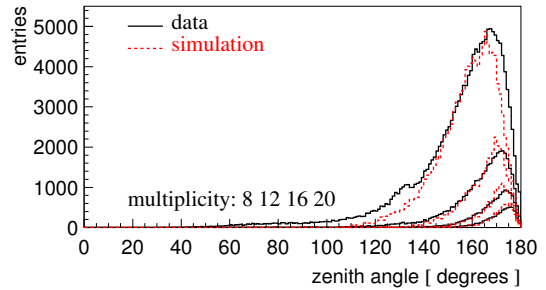
Figure 10. Muon zenith angle distribution of data and simulation
