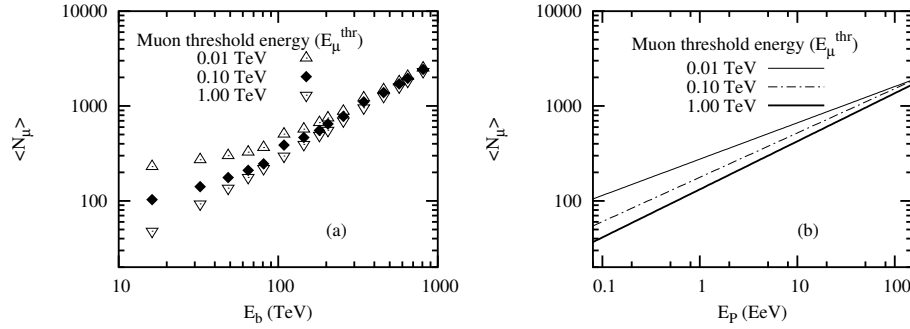
Figure 2. (a) Average muon number at the first interaction level versus bubble energy for different muon energy thresholds. (b) Variation of average number of muons with primary energy of cosmic rays particle at the first interaction level for different muon threshold energies and for the fraction of energy transfer f_e = 0.3 . Data is taken from 5000 proton induced showers.
