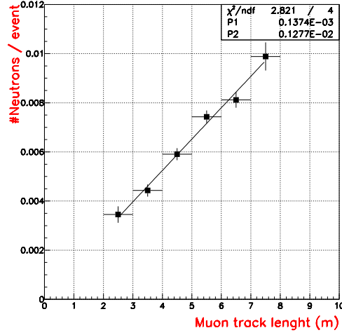
Figure 3. Number of neutrons per events detected as a function of the muon track length in scintillator; the main production of neutron is due to the muon interaction with the detector nuclei.
