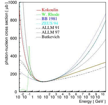
Figure 3. Photon-nucleon cross sections. Curves 5-7 are calculated according to \sigma_{\gamma N} = \lim_{Q^2 \rightarrow 0} \frac{4\pi^2 \alpha F_2^N}{Q^2}
