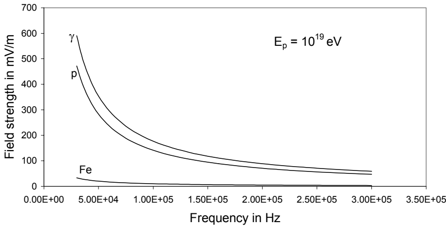
Figure. 2 Frequency spectra of vertical component of Field strength
