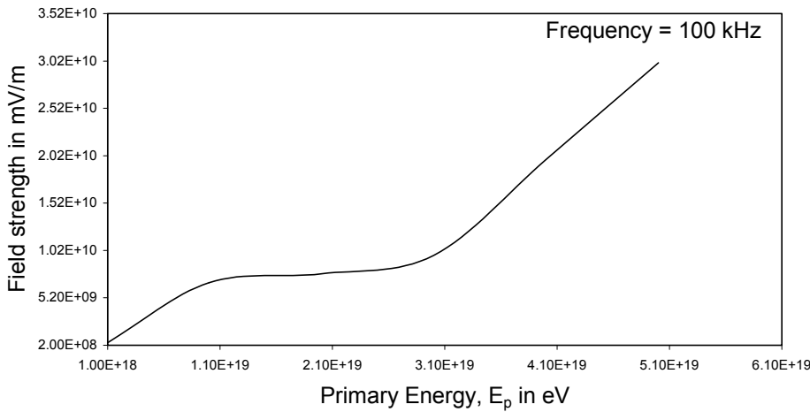
Figure 3. Variation of vertical component of Field strength with Primary Energy E_p for proton initiated shower.
