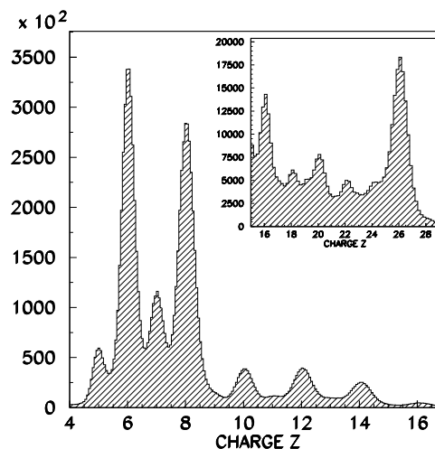
Figure 2. Charge histogram for all events measured in flight.
