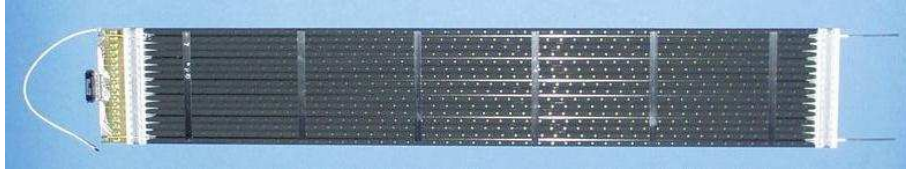
Figure 2. An AMS TRD straw tube module
