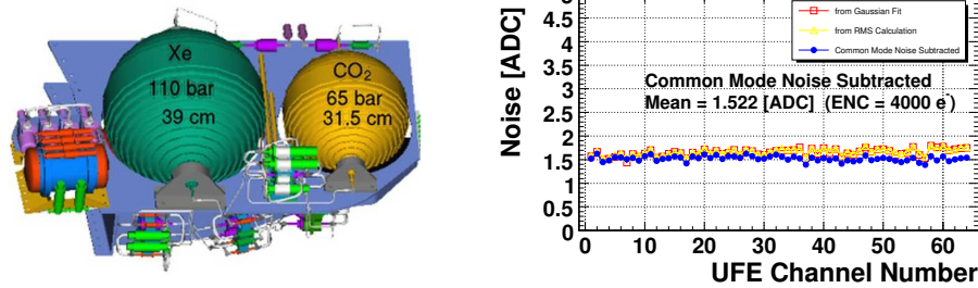
Figure 4. The TRD gas supply system ( left ), common mode subtracted noise distribution of a front end board serving 4 modules with 16 channels each ( right )
