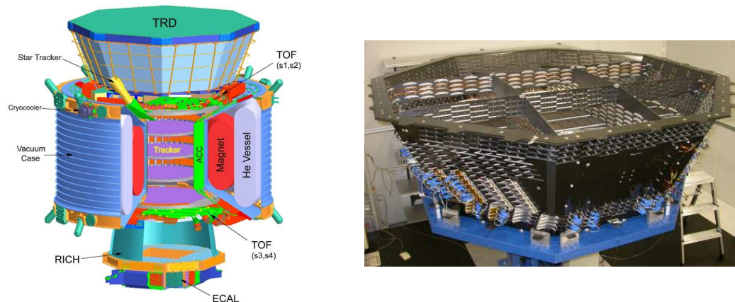
Figure 1. Schematic view of the AMS-02 experiment with the TRD on top ( left ), AMS-02 TRD support structure on the assembly stand during module integration ( right )
