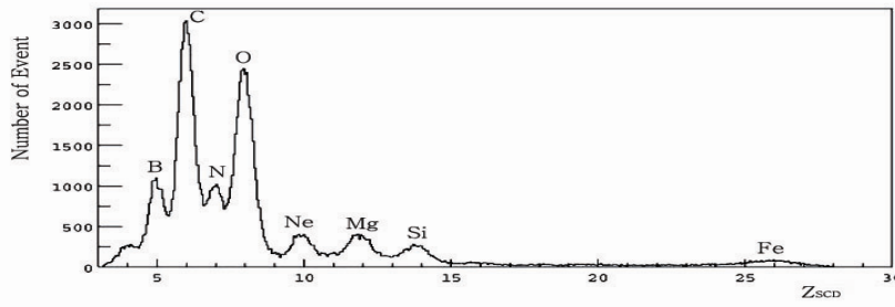
Figure 4. SCD Charge spectrum by the projection of high energy signals in Figure 3. The relative abundances are not corrected here.
