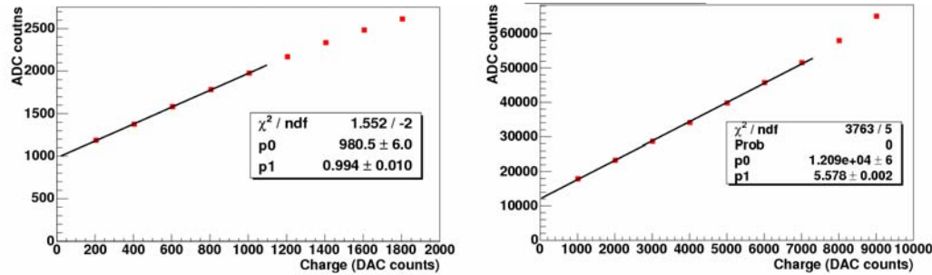
Figure 5. (a) Charge calibration run averaged over 32 channels of a VA chip, linear up to ~2100 ADC counts (~1 pC); (b) charge calibration run averaged over 16 channels of a CR chip, linear up to ~40000 ADC counts (~4 pC).
