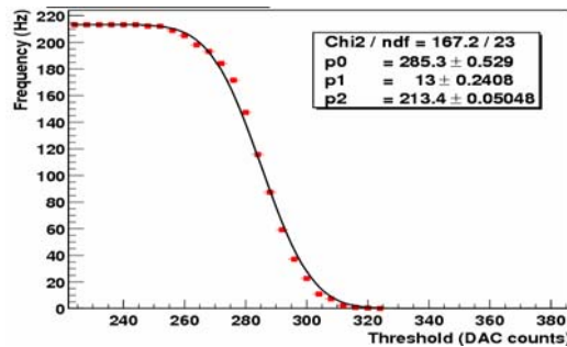
Figure 6. Trigger gain measurement for a typical channel of a VA/TA chip with a charge input of 100 DAC counts (~0.1 pC), showing a gain of about 2.85 DAC/ADC.
