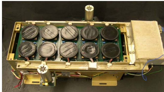
Figure 1. Calorimeter HPD box with EN-4/EN-11 HV potting
