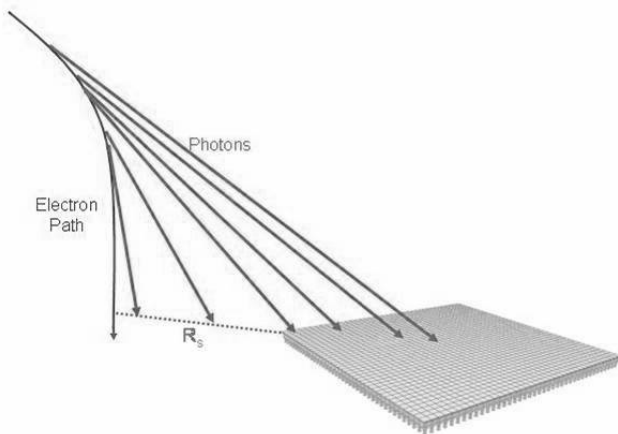
Figure 2. CREST detection concept. The effective area, R_s , of the detector is much larger than the actual physical size of detector.
