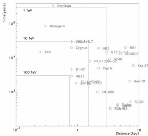
Figure 1. Distance and age of nearby SNRs and pulsars (Compilation by Swordy [2]).
