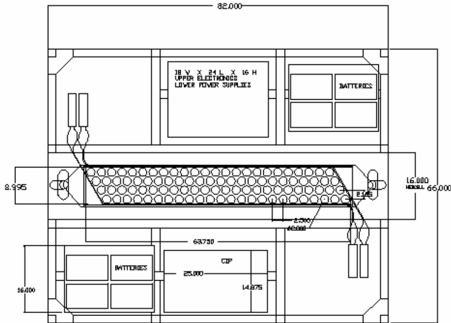
Figure 3. The CREST-1 instrument (dimensions in inches)
