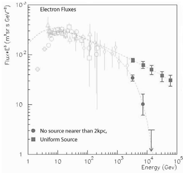
Figure 4. Electron flux spectrum
