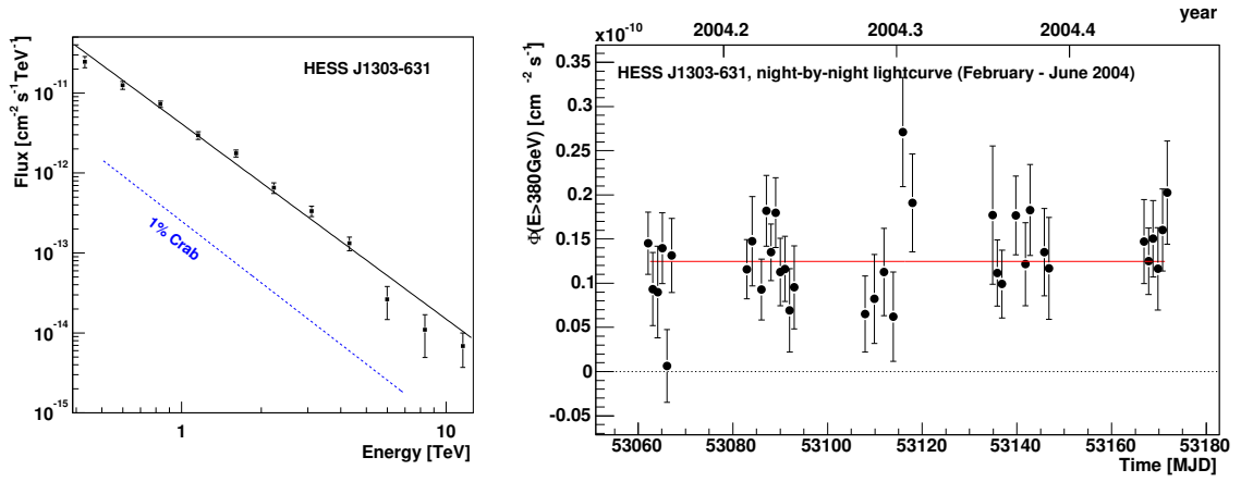
Figure 2. Left: The differential energy spectrum of HESS J1303-631. A fit to the data with a power law (solid line) is shown. The power-law corresponding to a spectrum of 1 % of the Crab Nebula is also indicated (dashed line). Right: The HESS J1303-631 light curve covering February until June, 2004. Shown is the integral flux \Phi(E > 380 \text{ GeV}) vs. time in night-by-night bins. The fit of a constant function (solid line) results in a \chi^2/\text{d.o.f.} of 35/35 being compatible with constant emission.
