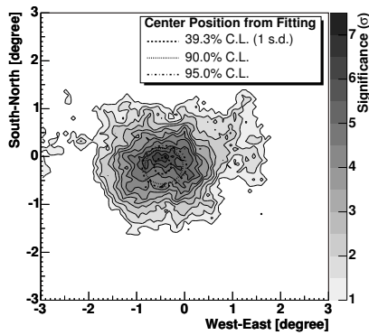
Figure 1. Source map and significance.
