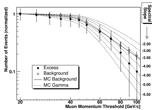
Figure 2. Number of excess events vs. energy threshold.
