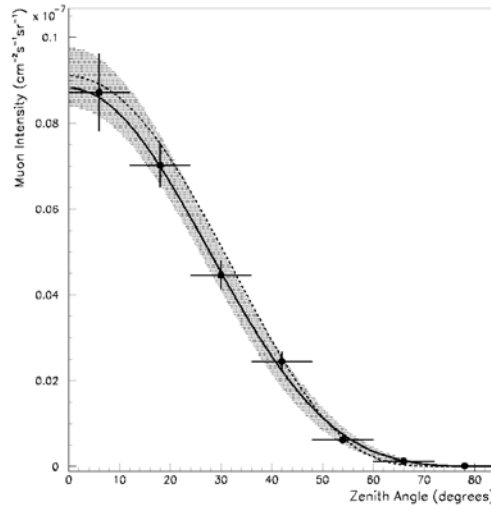
Figure1. Comparison of the measured atmospheric muon fluxes with results of fits. The solid points represent the data corrected for (pseudo)efficiencies in reconstructing tracks, as evaluated by a Blind Fit. The gray band represents the results of the fit within one sigma, the solid line represents the results of the Blind Fit and the dotted curve represents the solution using a parametrization.
