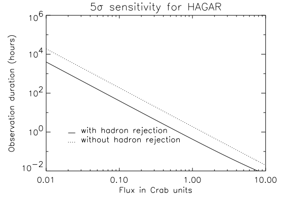
Figure 4. Sensitivity of HAGAR array ( \approx 7.7\sigma/\sqrt{\text{hour}} for 1 Crab)
