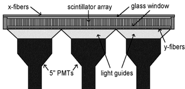
Figure 1. Detector plane element consisting of scintillator (in this case a segmented CsI array of 2 \times 2 mm 2 pixels produced by St. Gobain Crystals and Detectors) read out by crossed wavelength-shifting fiber arrays and multi-anode PMTs (not shown). The fibers are used for position determination. The large area PMTs are used for measuring total energy deposit.
