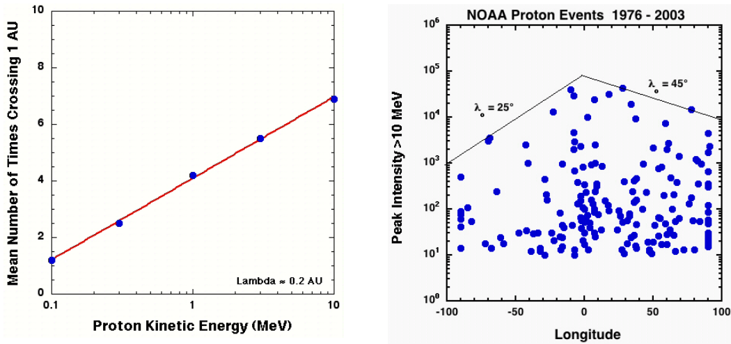
Figure 1. (Left) Plot of the average number of times solar protons pass outward across 1 AU as a function of energy (based on a simulation by Joe Giacalone assuming a mean free path of 0.2 AU). A logarithmic dependence was fit to these results and extrapolated to higher energy. (Right) Longitude distribution of large SEP events observed by the NOAA GOES satellites from 1976-2003. The e-folding longitudes used in this study are indicated.
