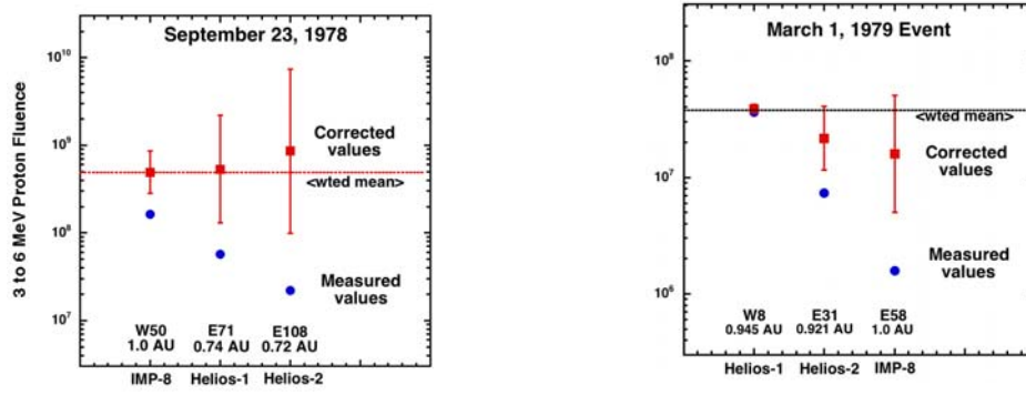
Figure 2. A comparison of the fluence of 3 to 6 MeV protons measured by Helios-1 & 2 and IMP-8 for the 9/23/78 and 3/1/79 events (based on measurements by Reames et al. [6]). The locations of the three spacecraft relative to the flare site are indicated. Once corrected for latitude and radius, the three estimates are in reasonable agreement.
