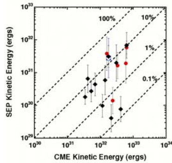
Figure 3. A comparison SEP and CME kinetic energies for 17 SEP events including the 21 April 2002 event (open square), the five events from October-November 2003 (circles) and 11 other events observed from 1998-2003.
