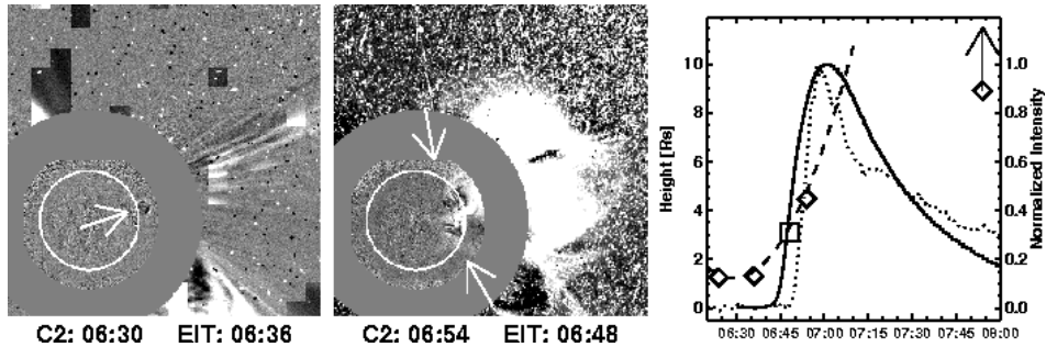
Figure 4. (left) SOHO’s LASCO (06:30) and EIT (06:36) difference images superposed. No CME in the LASCO image but the EIT image shows the early phase (arrow) of the 2005 January 20 CME. (middle) LASCO CME at 06:54 UT, with the overall extent of EUV disturbance at 06:48 UT (arrows). (right) CME height-time (diamonds with dashed line), GLE intensity (dotted lines) and GOES soft X-ray light curve (solid line). The square represents the inferred CME height from the EUV disturbance at 06:48 UT. The last LASCO height may be an underestimate due to ‘snow storm’.
