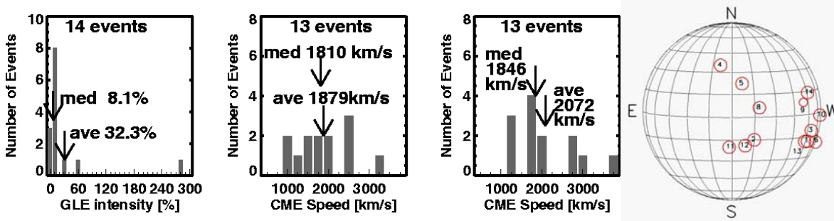
Figure 1. (left-to-right) GLE intensity, sky-plane speed of CMEs, space speed of CMEs and the solar sources. The mean and median values of the distribution are shown. The outlier in the intensity distribution is the 2005 January 20 CME.
