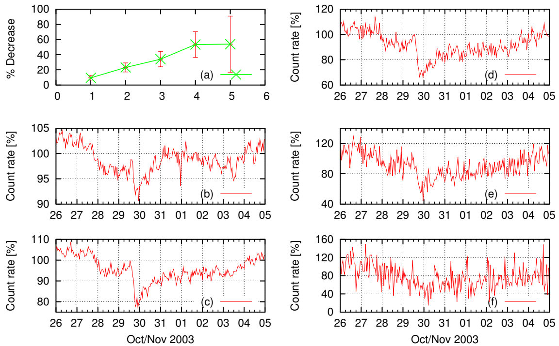
Figure 2. (a) % Decrease in neutron bunches as one moves from bunch-1 to bunch-5. Plots (b,c,d,e,f) show variation in the neutron Bunch countrate from October 26 to November 5 overlapping the occurrence of a X17/4B class Solar flare with onset at 9:51 Hrs UT on 28 October.
