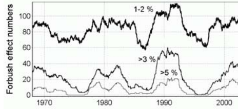
Figure 3. 729 day running sum for number of Forbush effects with different magnitude.
