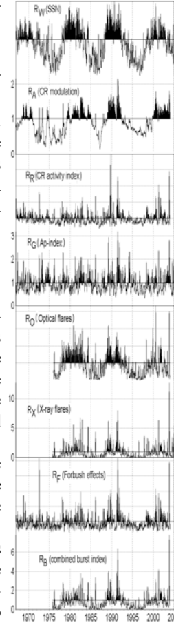
Figure 5. Different burst indices.
