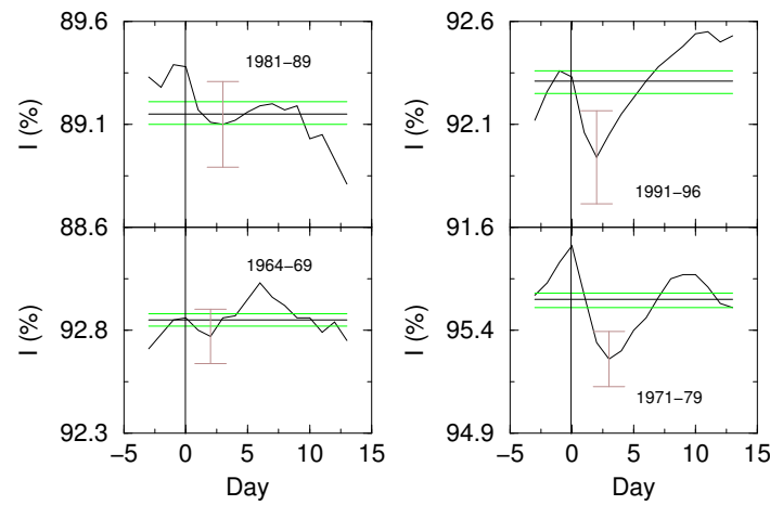
Figure 4. Mean superposed intensity along with the 95% confidence interval for minimum intensity (vertical bar) and for mean intensity (upper and lower horizontal bars) along with the mean counts (middle horizontal bar) in different solar epochs.
