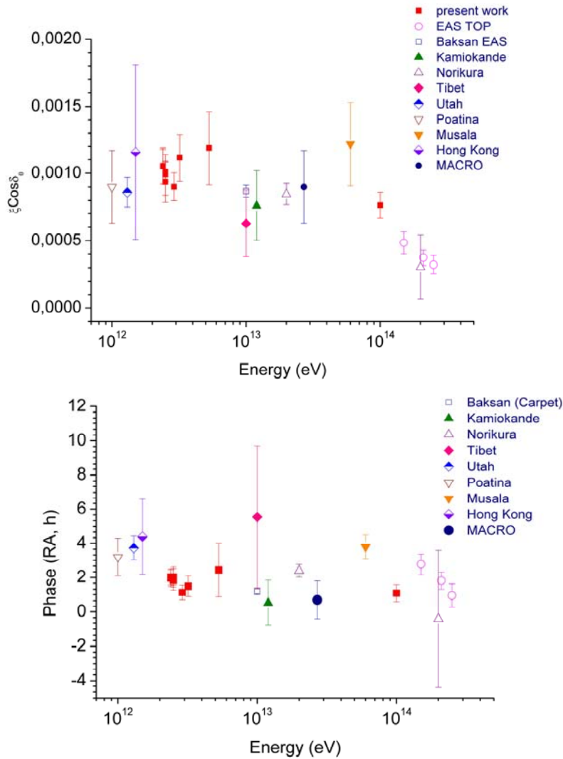
Figure 3. Energy dependence of the amplitude (reduced to the equator) and phase of the first harmonic of cosmic ray intensity in sidereal time.
