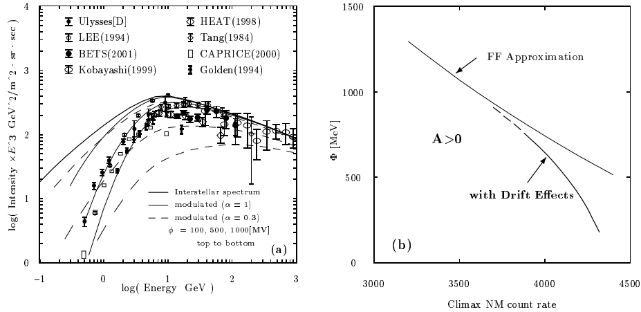
Figure 2. (a) Expected electron modulated spectra with the energy dependence of diffusion coefficient of 0.3, 1. \phi [MV] represents the parameter including the boundary of solar magnetosphere and the solar wind speed and is related with the energy part of the diffusion coefficient D_2(E) of \Phi \sim (p/D_2)\phi . (b) The \Phi - N relationship: The thin curve represents the FF approximation at the response energy 11GeV of the neutron monitor[8], while the thick curve is an expected \Phi - N curve of electrons from the drift model in the solar quiet period of A > 0 , which is just estimated qualitatively.
