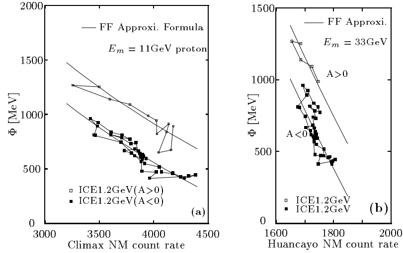
Figure 1. (a) The correlations between the modulation parameter \Phi [MeV] and the Climax neutron monitor count rate N . ICE 1.2 GeV electron data[3] are estimated from the LIS shown in Fig.2(b). The thin curves show 11GV proton curves of FF approximation formula[8] with N_{max} = 5000, 5800 . (b) Similarly shown in the case of Huancayo neutron monitor. The curves show 33GV proton curves with N_{max} = 1900, 2000 .
