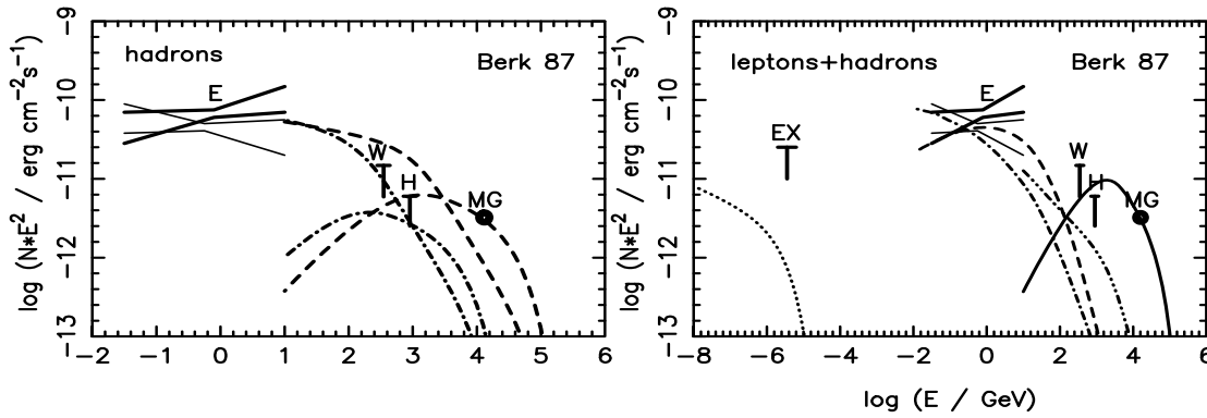
Figure 2: The multiwavelength spectrum observed from the region toward the open cluster Berk 87: the EX-OSAT satellite (marked by EX, Warwick et al. 1988), the unidentified EGRET sources from the 3rd Catalog 3EG 2016+3657 (thin solid) and 3EG J2021+3716 (thick solid) (E, [10]), the Whipple upper limit (W, [8]), the HEGRA upper limit (H, [2]), and the Milagro detection of the extended source MGRO J2019+37 (MG, filled circle [1]). \gamma -ray spectra produced by hadrons interacting with the matter inside the open cluster with density 10 \text{ cm}^{-3} and with the matter of the surrounding molecular clouds with density 10^4 \text{ cm}^{-3} (left figure). Hadrons are injected with the power law spectrum with the spectral index 2.1 and the high energy cut-off obtained for the magnetic field 10^{-4} \text{ G} (dashed curves) and 10^{-5} \text{ G} (dot-dashed curves). The energy conversion efficiency into relativistic particles is \eta_p = 3 \times 10^{-3} . The capturing factor of hadrons by the surrounding massive clouds is \xi = 10\% (dashed spectra) and 4\% (dot-dashed spectra). The comparison with the photon spectra produced by electrons in the synchrotron (dotted curve), IC (dashed) and bremsstrahlung (dot-dashed) processes and the \gamma -ray spectra from decay of \pi^0 produced by hadrons in collisions with the matter with density 10 \text{ cm}^{-3} inside the open cluster (triple dot-dashed curve) and hadrons which escaped from the open cluster into the surrounding molecular clouds with density 10^4 \text{ cm}^{-3} (solid curve) (right figure). Both, electrons and hadrons, have the power law spectrum (spectral index 2.4) and the high energy cut-offs determined by the magnetic field 10^{-5} \text{ G} . It is assumed that electrons and hadrons take a part \eta_e = 5 \times 10^{-3} and \eta_p = 10^{-3} of the power of the WR star wind. All hadrons escaping from the open cluster are captured by molecular clouds. The density of radiation is described by \mu = 1 .
