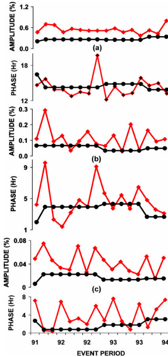
Fig 1: Amplitude and phase of the (a) diurnal, (b) semi-diurnal and (c) tri-diurnal anisotropy for HAEs along with the quiet day annual average values during the period 1991-94.
