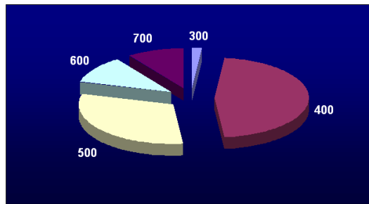
Fig 2 : The pie diagram of the solar wind velocity for all HAEs.
