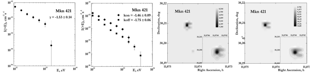
Figure 2: left – The Mkn 421 \gamma -quantum integral spectrum with power index of k_\gamma = -1.53 \pm 0.14 ; The event spectrum from Mkn 421 with background with index of k_{ON} = -1.46 \pm 0.09 and spectrum of background events observed simultaneously with Mkn 421 with index k_{OFF} = -1.75 \pm 0.06 ; right – The Mkn 421 image at energy range of > 0.8 TeV; and The energy image (in TeV units) of Mkn 421 by SHALON.
