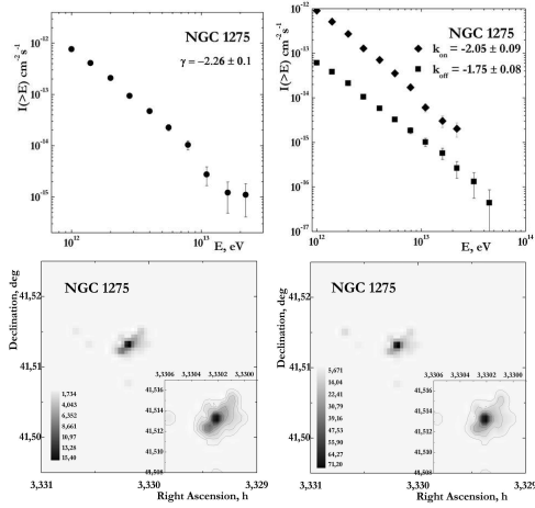
Figure 6: top: left – The NGC 1275 \gamma -quantum integral spectrum with power index of k_\gamma = -2.26 \pm 0.10 ; right – The event spectrum from NGC 1275 with background with index of k_{ON} = -2.05 \pm 0.09 and spectrum of background events observed simultaneously with NGC 1275 with index k_{OFF} = -1.75 \pm 0.08 ; bottom: The NGC 1275 image at energy range of > 0.8 TeV; and The energy image (in TeV units) of NGC 1275 by SHALON.
