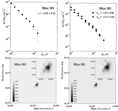
Figure 4: top: left – The Mkn 501 \gamma -quantum integral spectrum with power index of k_\gamma = -1.85 \pm 0.11 ; right – the event spectrum from Mkn 501 with background with index of k_{ON} = -1.83 \pm 0.06 and spectrum of background events observed simultaneously with Mkn 501 with index k_{OFF} = -1.72 \pm 0.06 ; bottom The Mkn 501 image at energy range of > 0.8 TeV; and The energy image (in TeV units) of Mkn 501 by SHALON.
