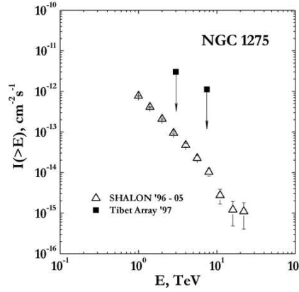
Figure 5: The NGC 1275 gamma - quantum ( E > 0.8 TeV) integral spectrum by SHALON in comparison with Tibet Array data [12];
