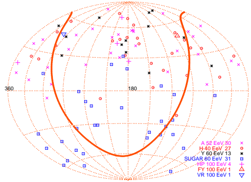
Figure 1: Skymap of the UHECR arrival directions of events with rescaled energy E' > 4 \times 10^{19} eV in equatorial coordinates; magenta crosses—30 Agasa (A) events with E > 5.2 \times 10^{19} eV, red circles—27 HiRes (H) events with E > 4 \times 10^{19} eV, black stars—13 Yakutsk (Y) events with E > 6 \times 10^{19} eV, blue boxes—31 Sugar (S) events with E > 6 \times 10^{19} eV, magenta crosses—4 Haverah Park (HP) events with E > 10^{20} eV, red triangle—one Flye's Eye (FY) event with E > 10^{20} eV, blue triangle—Volcano Ranch (VR) event with E > 10^{20} eV.
