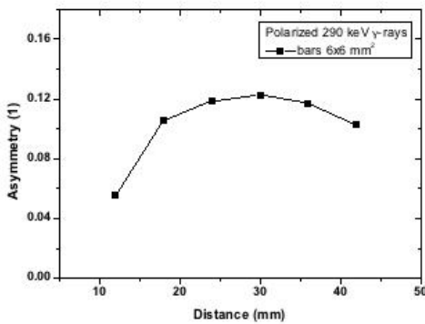
Figure 5: Measured level of asymmetry up to 12%, as a function of distance between bars triggering coincident hits.
