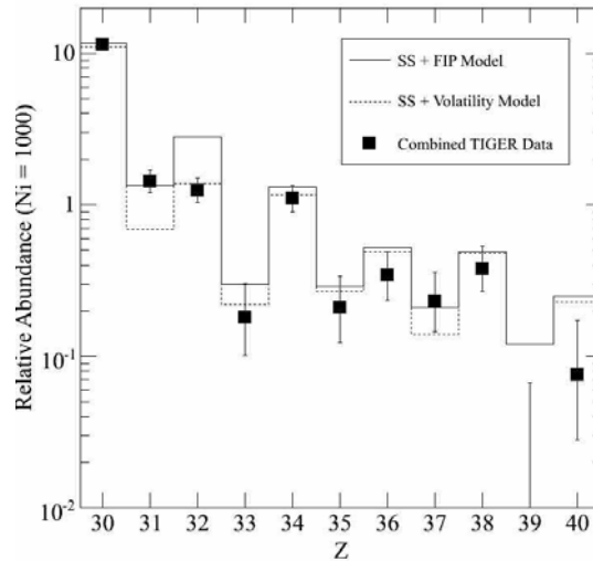
Figure 3: Relative abundances observed at the TIGER instrument, compared with results of propagating two possible source models to the balloon's atmospheric depth.
