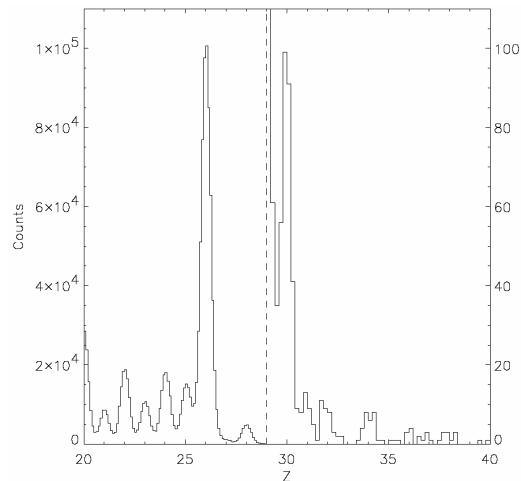
Figure 1: Charge histogram of combined dataset from 2001 and 2003 flights
