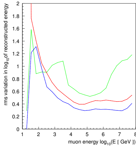
Figure 2: Energy reconstruction precision: blue (lowest curve) for the photon-density-based approach of this paper, red for the Q_{tot} and green (highest curve) for the N_{ch} -based calculations.
