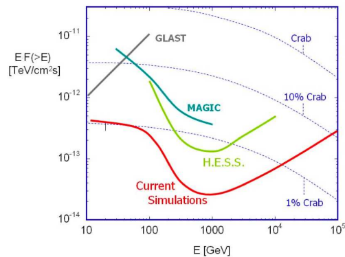
Figure 1: This figure illustrates roughly the sensitivity that can be achieved with an array of Cherenkov telescopes as CTA. The exact values will finally depend on the real layout of the system.
